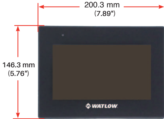
Overall dimensions
