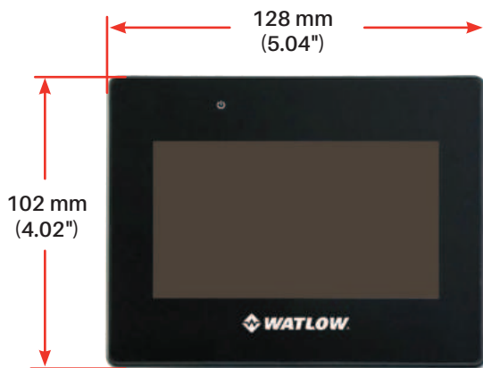
Overall dimensions
