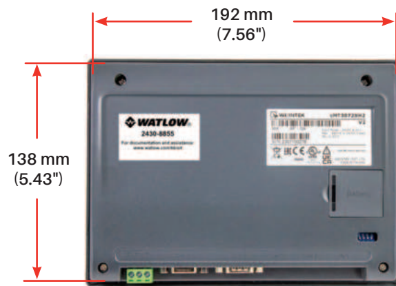
Panel cut-out dimensions
