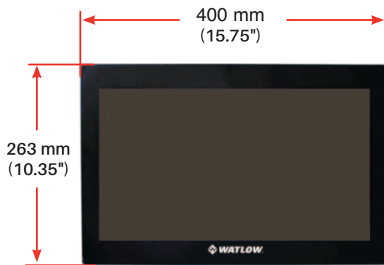
Overall dimensions
